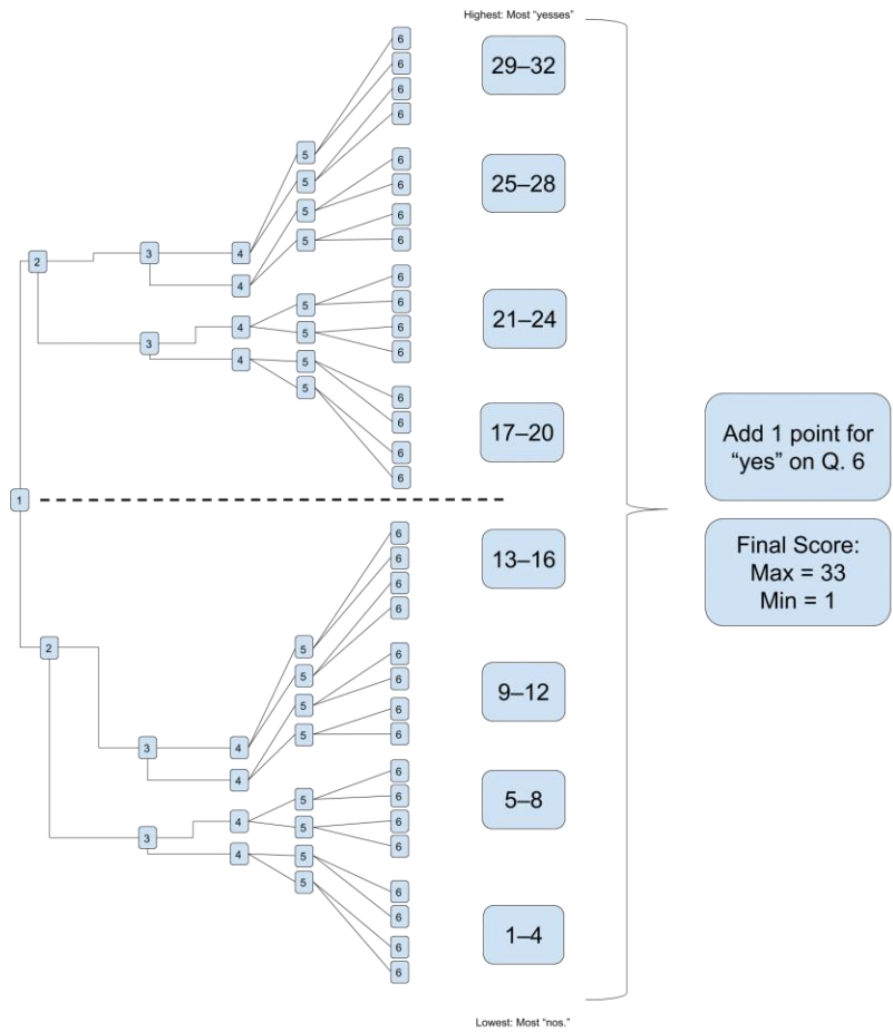
Illustration of HET's Branching Structure
